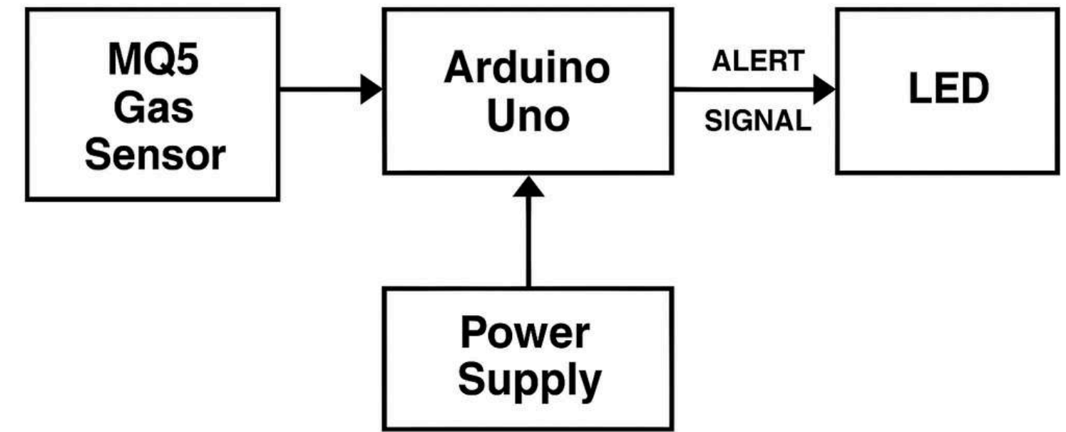
Block Diagram
